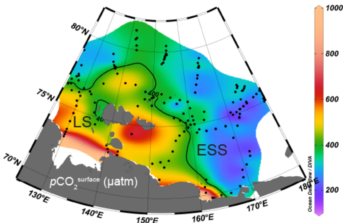
Figure 9. \text{pCO}_2 in the surface waters of the Laptev Sea (LS) and East Siberian Sea (ESS) as observed in 2008 and 2014. The isoline of 400 \mu\text{atm} indicates the atmospheric level.
