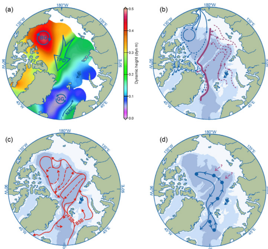
Figure 4. Schematic representations of Arctic Ocean circulation: (a) Surface circulation of the Arctic Ocean as shown by dynamic topography (20/400 dbar) (World Ocean Database 2013), (b) summary of mid-water halocline sources, flows and associated fronts (blue shows Pacific-origin waters, maroon shows Atlantic-origin waters, thick maroon line depicts the front between them) after McLaughlin et al. [1996]; (c) schematic representation of the Arctic Circumpolar Boundary Current system derived from Atlantic water inflows [after Aksenov et al. , 2011; Rudels et al. , 2013]; and (d) schematic representation of deep water exchange [Aagaard et al. , 1985]. BG is the Beaufort Gyre, BSB is the Barrents Sea Branch, FSB is the Fram Strait Branch, GG is the Greenland Gyre, NAC is the Norwegian-Antarctic Current, NCC is the Norwegian Coastal Current, TPD is the Transpolar Drift. [Figure copied from Blum et al. , 2015.]
