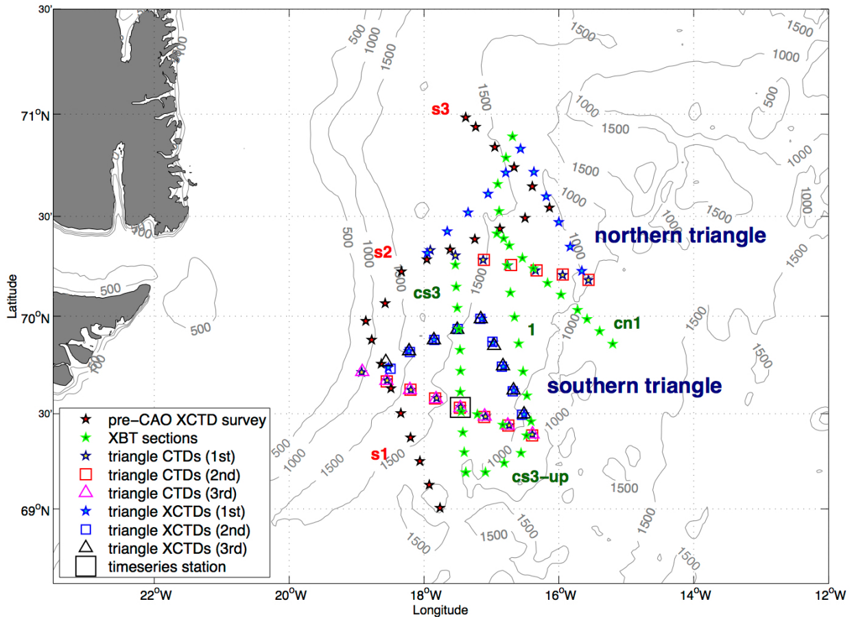
Figure A2: Detailed shipboard sampling done in the northwest Iceland Sea (within the boxed region of figure A1). See the legend for an explanation of the measurements.
