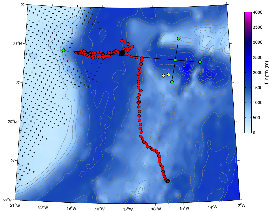
Figure 1: Glider track. The red circles mark the dives of the glider from 13 Feb to 18 March. The black lines are the nominal transects along which the glider operated. The yellow circles mark the UiB mooring and met buoy. The black dots indicate ice concentration in excess of 50% on 27 Feb.
