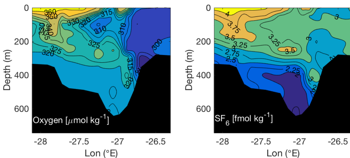
Figure. 2. Oxygen and SF 6 in the Denmark Strait during the IGP cruise.
