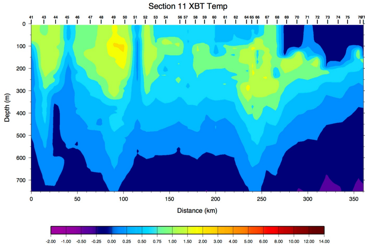
Figure A4: Vertical section of temperature ( ^{\circ}\text{C} ) for XBT transect 11 (see Fig. A1 for the location of the transect). The viewer is looking to the east. The station locations are indicated along the top of the plot.
