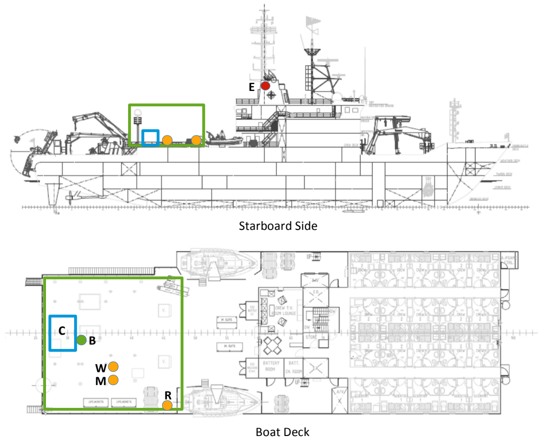
Figure 1. Locations of instruments: C: Container, B: Balloon Basket, R: HATPRO Radiometer, W: Windcube, M: Micro Rain Radar, E: Exhaust Stack.
