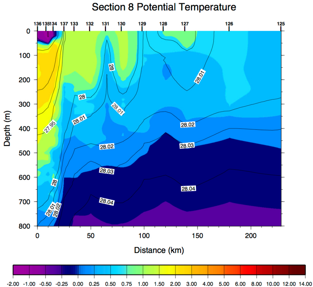
Figure A3: Vertical section of potential temperature ( ^{\circ}\text{C} , color) and potential density ( \text{kg m}^{-3} , contours) for transect 8 in the western Greenland Sea (see Fig. A1 for the location of the transect). The viewer is looking north. The station locations are indicated along the top of the plot.
