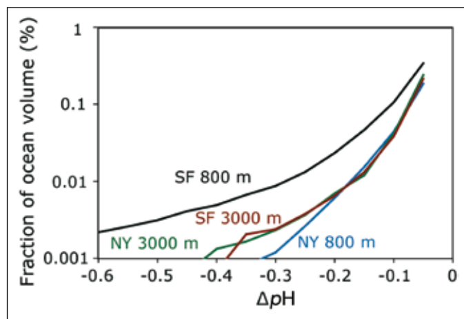
Figure 6.14 Estimated volume of pH perturbations at basin scale (Wickett et al. , 2003). Simulated fraction of global ocean volume with a \Delta\text{pH} less than the amount shown on the horizontal axis, after 100 years of simulated injection at a rate of 0.37 \text{ GtCO}_2 \text{ yr}^{-1} ( = 0.1 \text{ GtC yr}^{-1} ) at each of four different points (two different depths near New York City and San Francisco). Model results indicate, for example, that injecting \text{CO}_2 at this rate at a single location for 100 years could be expected to produce a volume of sea water with a \Delta\text{pH} < -0.3 units in 0.01% or less of total ocean volume (0.01% of the ocean is roughly 10^5 \text{ km}^3 ). As with other simulations of direct \text{CO}_2 injection in the ocean, results for the upper ocean (e.g., 800 m) tend to be more site-specific than are results for the deep ocean (e.g., 3000 m).
