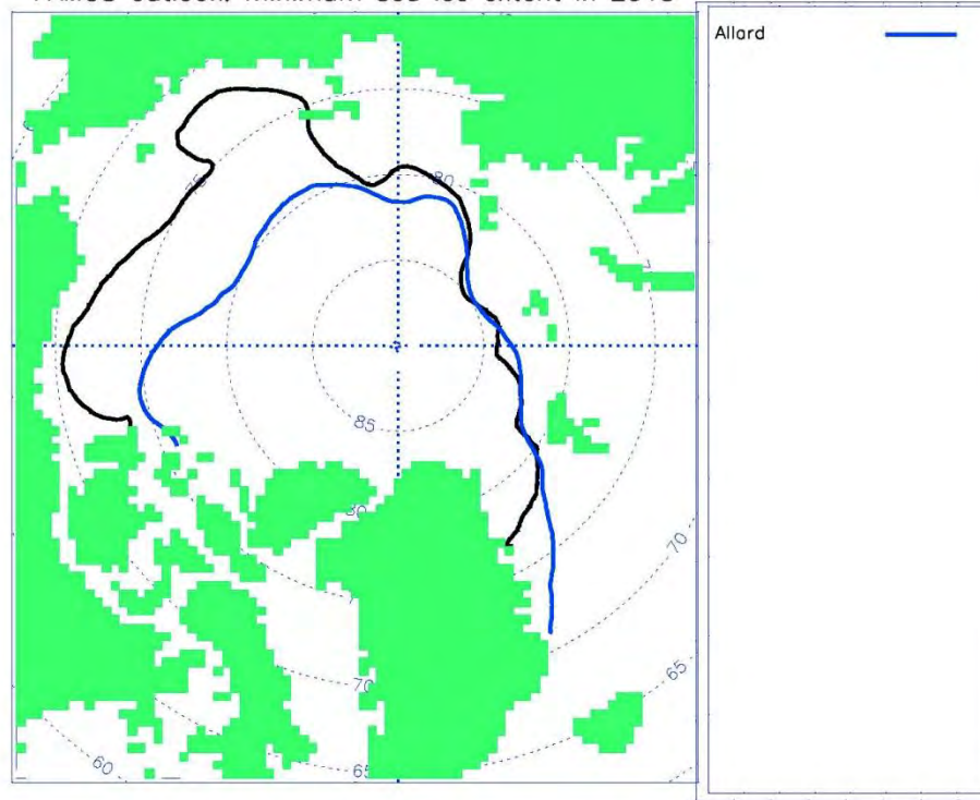
FAMOS outlook: minimum sea ice extent in 2013
